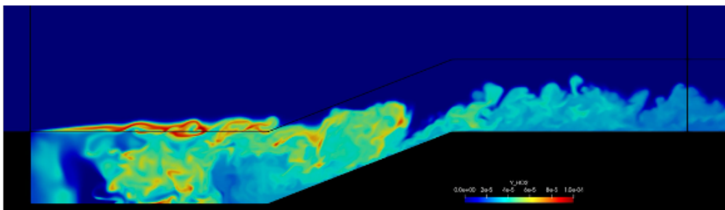
Figure 1: Instantaneous flame location shown via HO 2 mass fraction for a cavity scramjet
