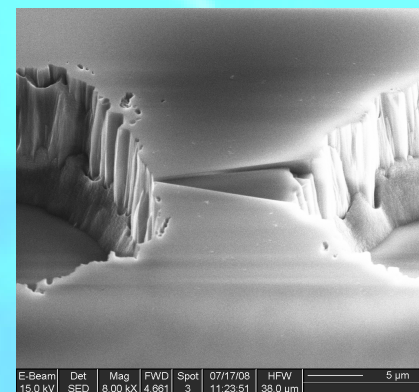
8V, 50KHz – nDEP
